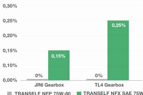
Renault B-SUV - Fuel Economy benefit on WLTC cycle
