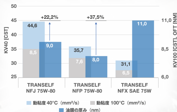
Viscosity vs. Oil Film Thickness
